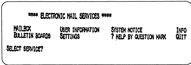
Main menu of FIMNET e.mail service, either in Finnish or English
